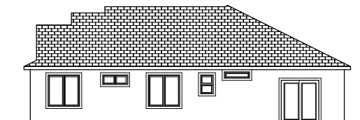
Back Elevation
